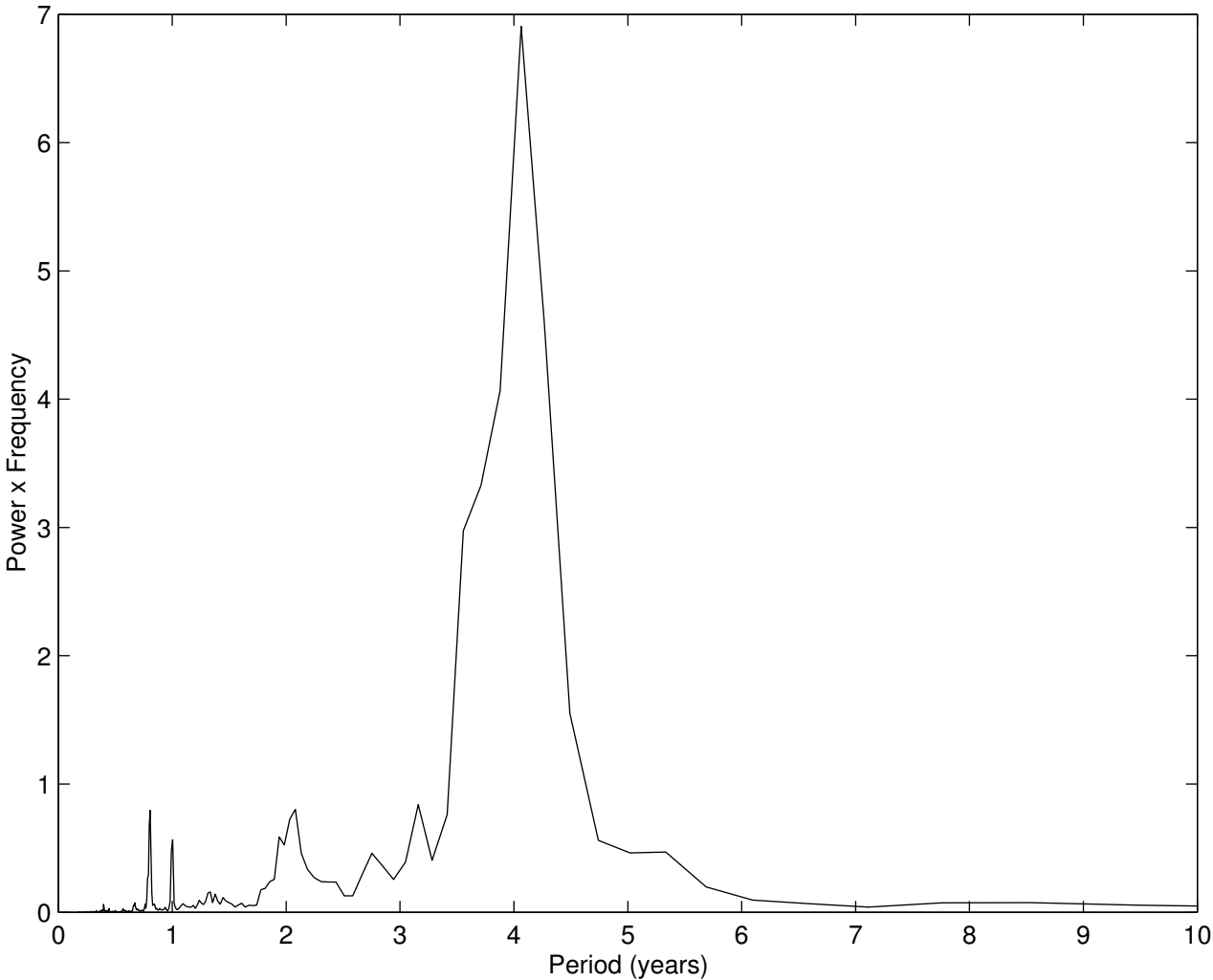
Power Spectrum of Nino 3 SST anomaly
