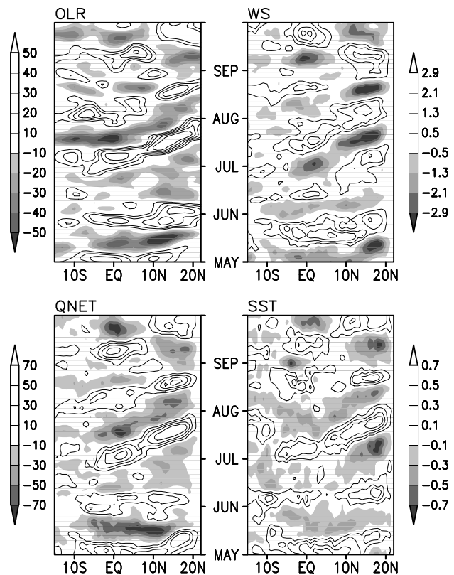
Figure 4. Time-latitude sections of 10-80 day filtered anomalies of OLR ( \text{W m}^{-2} ), windspeed ( \text{m s}^{-1} ), Q_{\text{net}} ( \text{W m}^{-2} ) and SST ( ^{\circ}\text{C} ) averaged over 85\text{-}90^{\circ}\text{E} in the summer of 1998.
