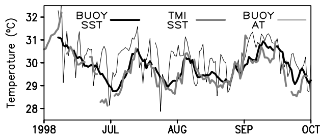
Figure 1. Evolution of daily buoy SST (bold), 3-day TMI SST (grey) and daily buoy air temperature (thin) at 18^{\circ}\text{N} , 88^{\circ}\text{E} in the north Bay of Bengal during summer 1998.
