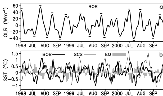
Figure 2. June-September 1998-2000 evolution of (a) 10-80 day filtered BOB OLR anomaly, with small bars (each of length 3 days) indicating dates used in the composites shown in Figure 3, and (b) SST anomaly averaged over BOB (bold), 15\text{--}20^{\circ}\text{N} , 115\text{--}120^{\circ}\text{E} (SCS, thin) and 2.5^{\circ}\text{S}\text{--}2.5^{\circ}\text{N} , 85\text{--}90^{\circ}\text{E} (EQ, shaded).
