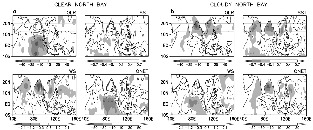
Figure 3. Composite structure of monsoon ISO in the (a) clear and (b) cloudy BOB phases. Anomalies of OLR ( \text{W m}^{-2} ), wind speed (WS; \text{m s}^{-1} ), Q_{\text{net}} ( \text{W m}^{-2} ) and SST ( ^{\circ}\text{C} ) are shown.
