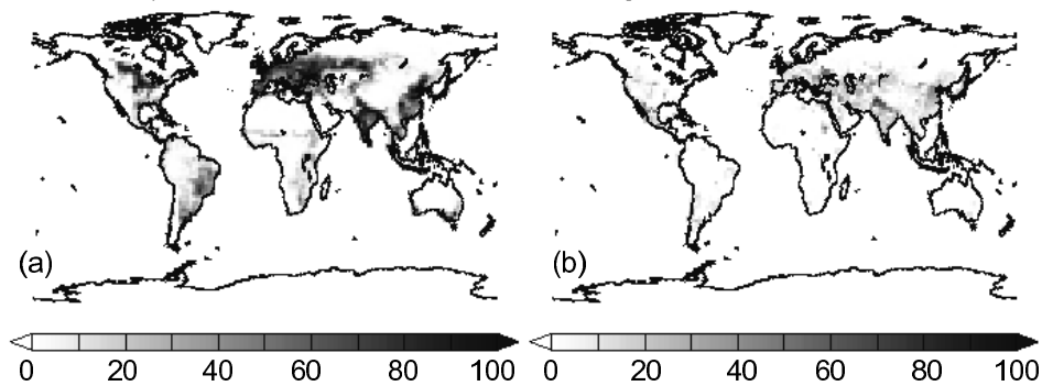
Figure 1. (a) The percentage of each 2.0^\circ \times 2.5^\circ grid cell defined as cropland within CAM3. (b) The estimated percentage of each 2.0^\circ \times 2.5^\circ equipped for irrigation [Doll and Siebert, 2000].
