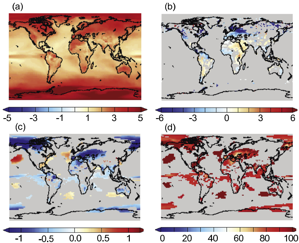
Figure 2. Annual average surface (a) temperature ( ^{\circ}\text{C} ) and (b) soil moisture (%) changes for doubled \text{CO}_2 in the absence of irrigation, [2 \times \text{CO}_2 - 1 \times \text{CO}_2]_{\text{no-irr}} . (c) Difference in temperature response to doubled \text{CO}_2 with and without irrigation, [2 \times \text{CO}_2 - 1 \times \text{CO}_2]_{\text{irr}} - [2 \times \text{CO}_2 - 1 \times \text{CO}_2]_{\text{no-irr}} . (d) Ratio (%) of same responses, [2 \times \text{CO}_2 - 1 \times \text{CO}_2]_{\text{irr}} / [2 \times \text{CO}_2 - 1 \times \text{CO}_2]_{\text{no-irr}} . Gray cells are not significant at p = 0.05 .
