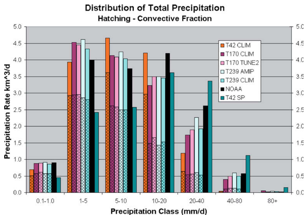
Fig. 13 The distribution of area-weighted precipitation rates as simulated by five versions of the CCM3 and in the NOAA gridded observational dataset. Also shown are results for the SP-CAM model (T42 SP), which is discussed in Sect. 4. The height of each bar is the total area-weighted precipitation rate (precipitation rate \times grid cell area) for daily events in each precipitation class (0.1–1 mm/day, 1–5 mm/day, etc.) The hatched section of each bar represents the amount of convective (as opposed to large-scale) precipitation. Simulated and observed precipitation data were averaged to the spatial grid of T42 ( \sim 300 km) before conducting the statistical analysis
