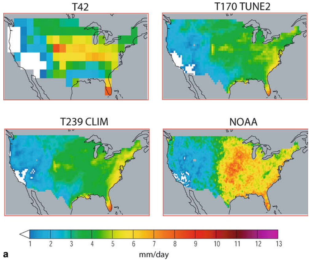
Fig. 8 a Mean daily precipitation intensities for the JJA season (precipitation on days having >0.1 mm of precipitation) as simulated by the CCM3 atmospheric model at spectral truncations of T42 ( \sim 300 km grid size), T170 ( \sim 75 km grid size), T239 ( \sim 50 km grid size) and in a gridded observational data set. Note that white signifies off-scale on the low end. b Same as a but with all datasets averaged to a T42 grid before statistics were calculated. Note that white signifies off-scale on the low end
