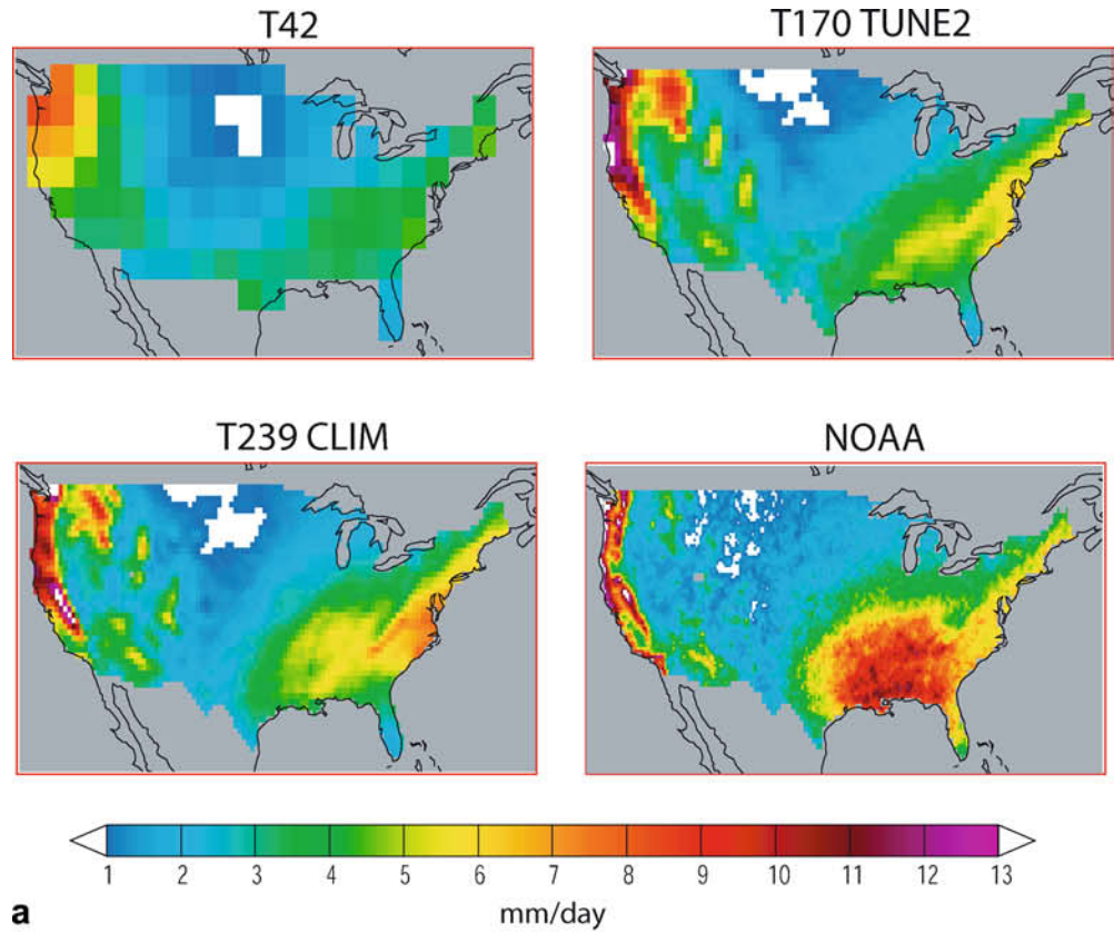
Fig. 9 a Same as Fig. 8a, but for the DJF season. Note that white signifies off-scale on the low end, except where seen along the west coast , where it signifies off-scale on the high end. b Same as Fig. 8b, but for the DJF season. Note that white signifies off-scale on the low end
