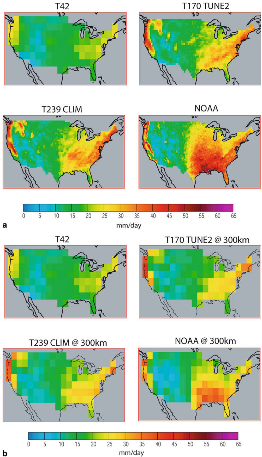
Fig. 10 a The 99 th percentile daily precipitation amounts, as simulated by the CCM3 atmospheric model at spectral truncations of T42 (~300 km grid size), T170 (~75 km grid size), T239 (~50 km grid size) and in the NOAA gridded observational data set. b Same as 10 but with all datasets averaged to a T42 grid
