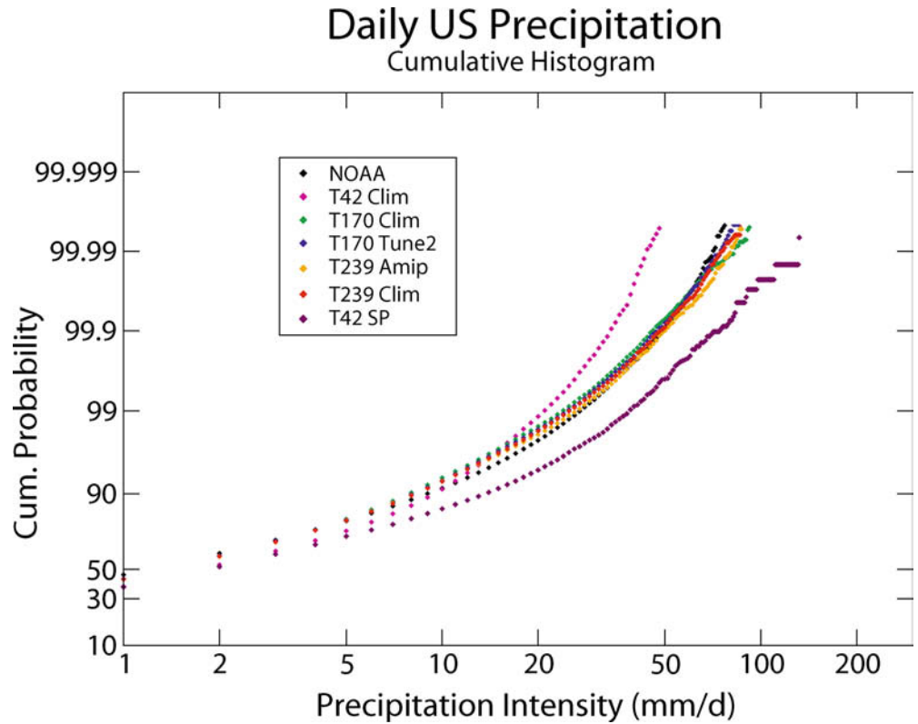
Fig. 11 Cumulative probability distribution for daily precipitation amounts in United States. Curves show the amount of daily precipitation (horizontal axis) of a given percentile (vertical axis). All precipitation data were averaged to the grid of the T42 mode prior to performing this analysis. Included with the CCM3 simulations is the result for the SP-CAM model (T42 SP), which is discussed in Sect. 4
