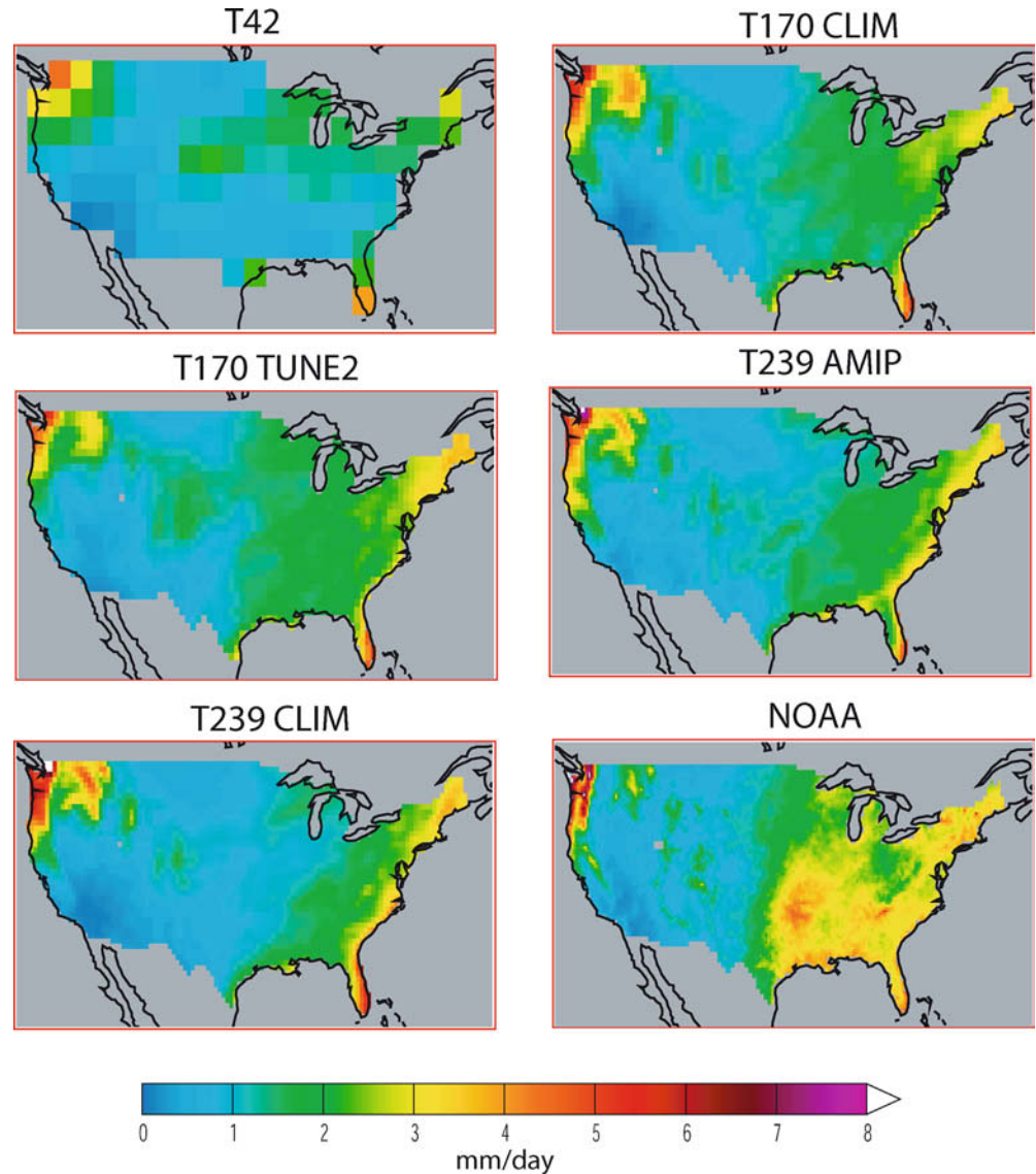
Fig. 5 The same as Fig. 1, except showing autumn (SON) precipitation. Note that white signifies off-scale on the high end
