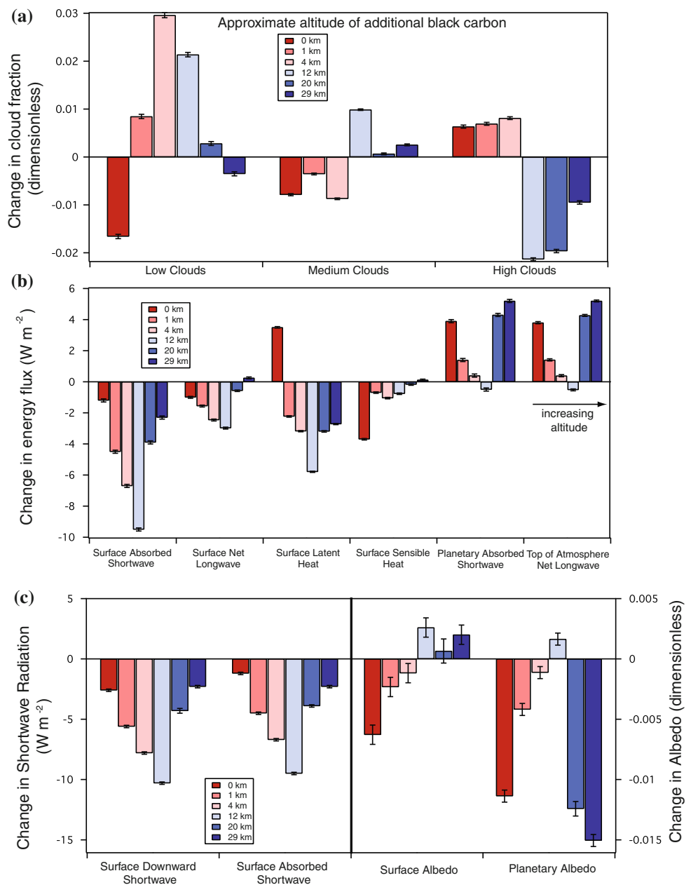
Fig. 5 Changes relative to the control for each simulation in a low, medium, and high clouds, b surface and top of atmosphere energy fluxes, and c surface downward and absorbed radiation, and surface and planetary albedo. Each simulation increases black carbon aerosol concentrations by 1 Mt at a different horizontal layer in the atmosphere. Approximate altitudes of layers with additional black carbon are indicated in the legend. Low clouds are those between the surface and \sim 3 km, medium clouds are between \sim 3 and \sim 7 km, and high clouds are above \sim 7 km. Longwave, sensible, and latent heat fluxes are positive upward; “surface absorbed shortwave” and “planetary absorbed shortwave” are equivalent to positive downward “surface net shortwave” and “top of atmosphere net shortwave,” respectively. Uncertainty is given by the standard error computed from 70 annual means using the Student t test with 95% confidence interval. The standard error is corrected for autocorrelation (Zwiers and von Storch 1995)
