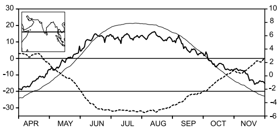
Figure 1. \Delta TT between the two boxes (thin solid, K \times 6 , the zonal extent of both boxes is between 30^\circ – 110^\circ E while the meridional extent of the northern (southern) box is between 10^\circ N – 35^\circ N ( 15^\circ S – 10^\circ N ), shown in inset), vertical shear of zonal wind (200 hPa–850 hPa) averaged over 50^\circ E – 90^\circ E , Eq.– 15^\circ N (dashed, m s^{-1} ) and latitude of zero absolute vorticity averaged between 50^\circ E and 100^\circ E (thick solid, right scale).
